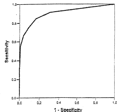
Receiver Operator Characteristics (ROC) curve for AD8
